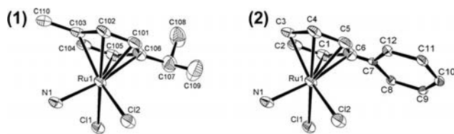
Figure 2. X-ray crystal structures of [(\eta^6\text{-}p\text{-cym})\text{Ru}(\text{NH}_3)\text{Cl}_2]\cdot\{(\text{dm}ba\text{-H})(\text{PF}_6)\} (1a) and [(\eta^6\text{-bip})\text{Ru}(\text{NH}_3)\text{Cl}_2] (2). Thermal ellipsoids show 50% probability. The hydrogen atoms have been omitted for clarity. The ion pair in 1a is not shown.
